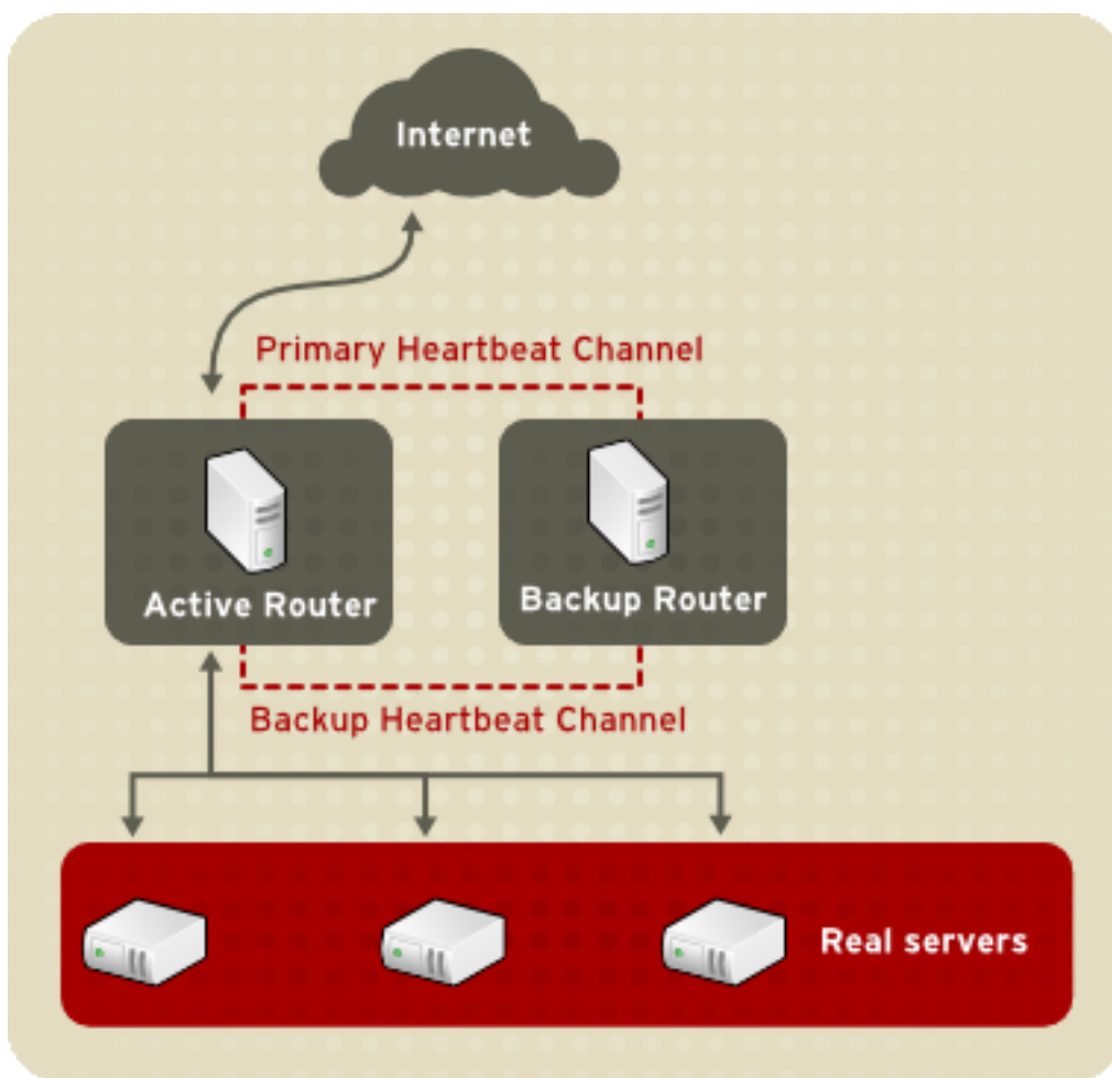
Figure 1.1. A Basic LVS Configuration
