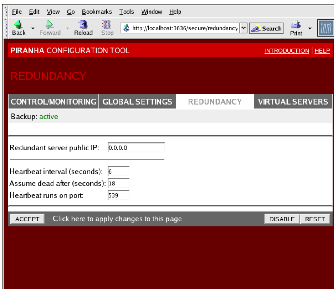
Figure 4.4. The REDUNDANCY Panel
