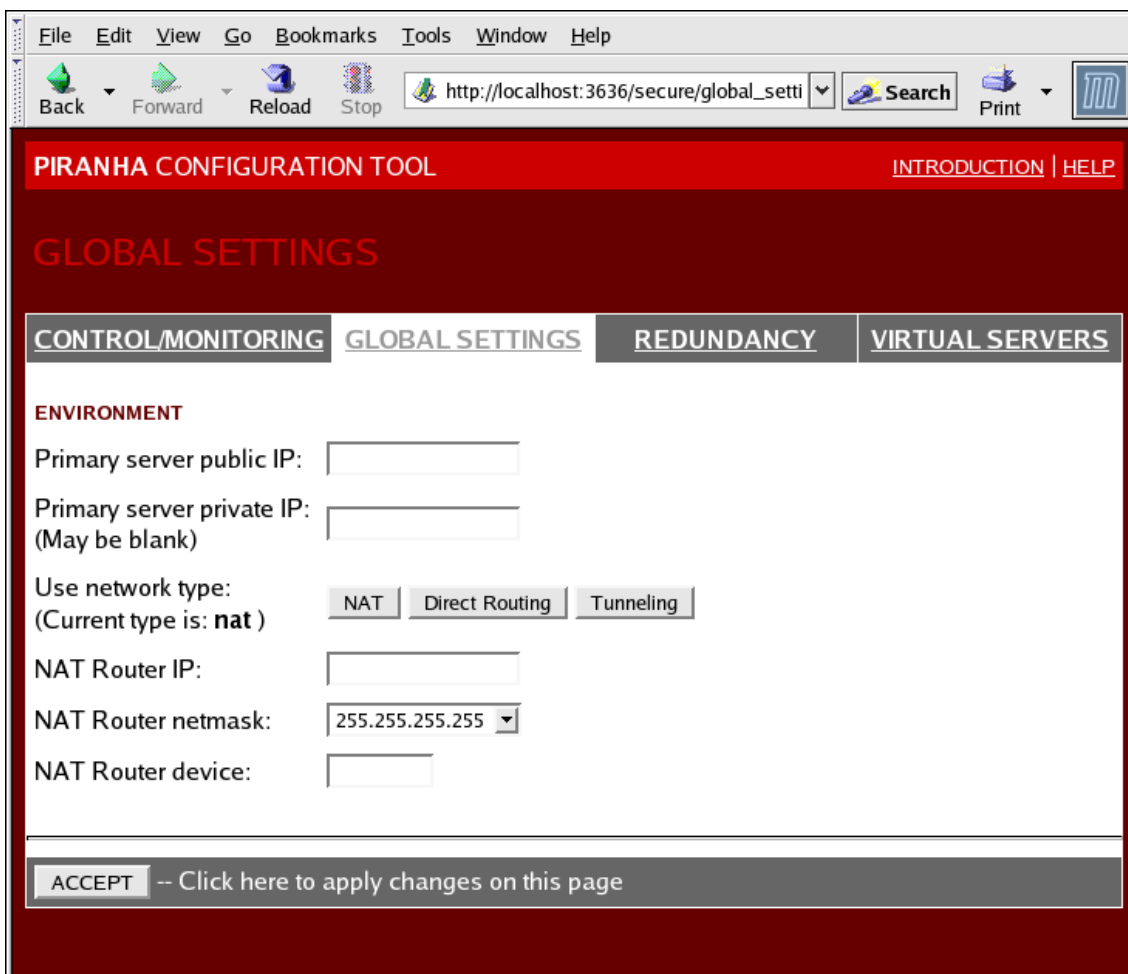
Figure 4.3. The GLOBAL SETTINGS Panel
