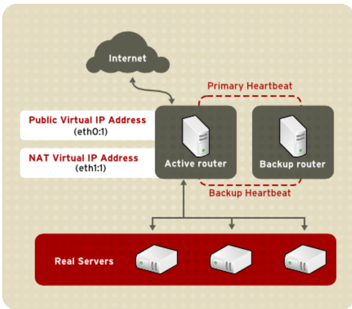
Figure 1.3. LVS Implemented with NAT Routing
