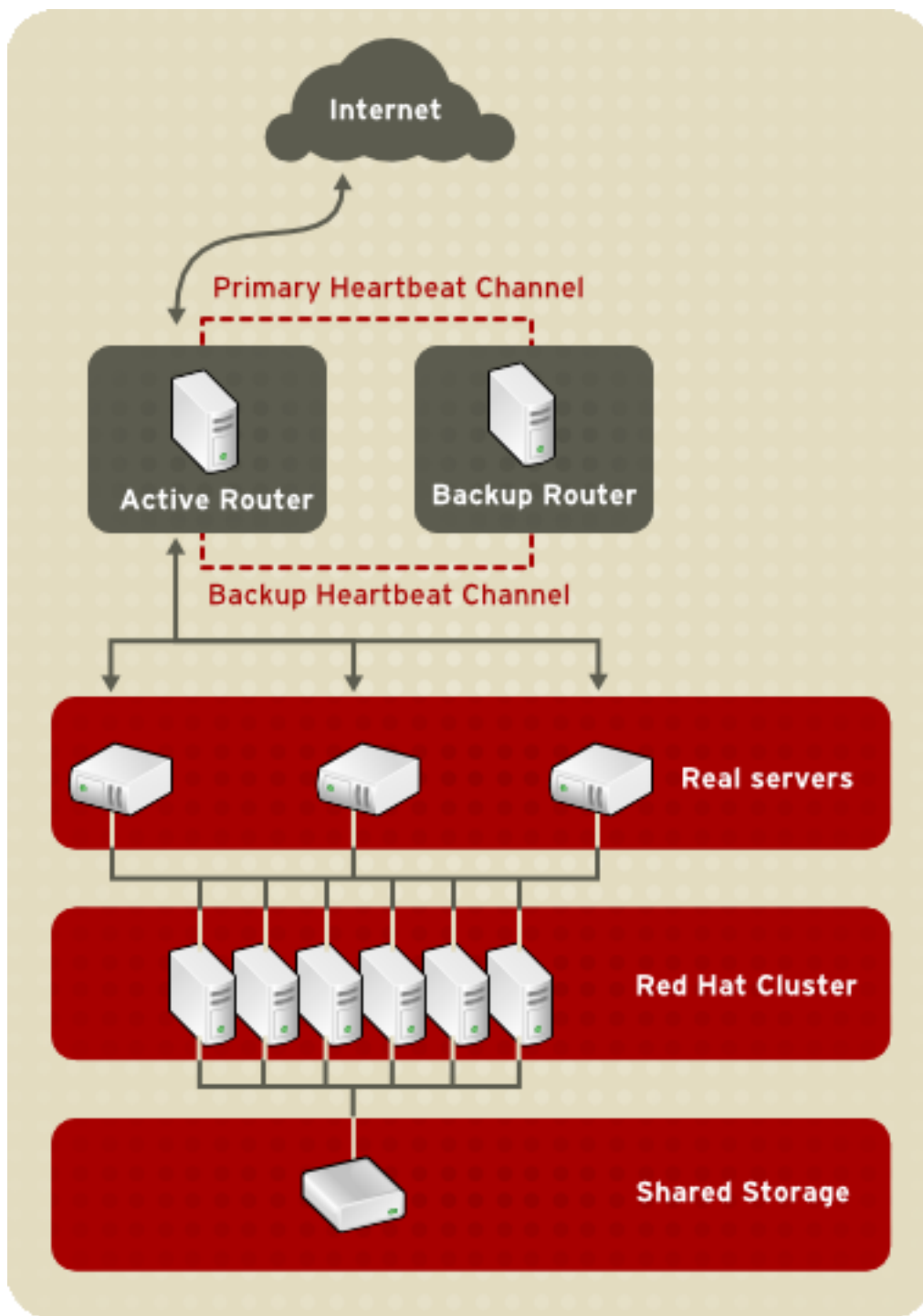
Figure 1.2. A Three-Tier LVS Configuration
