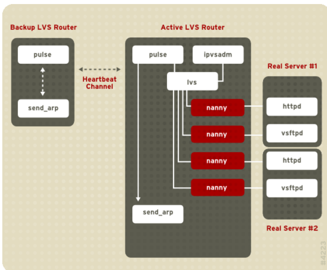
Figure 1.5. LVS Components
