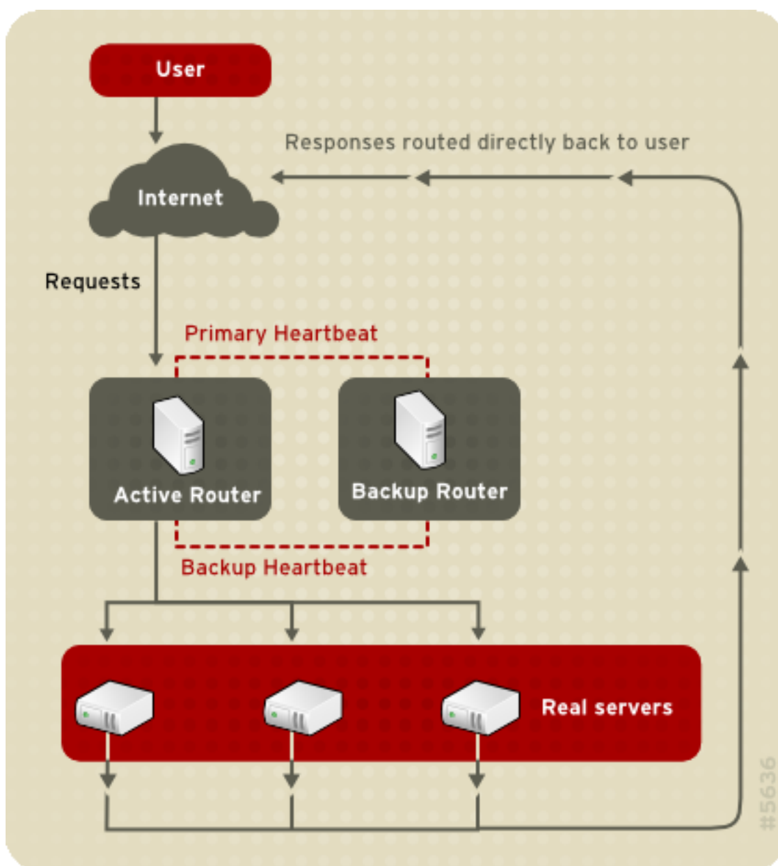
Figure 1.4. LVS Implemented with Direct Routing
