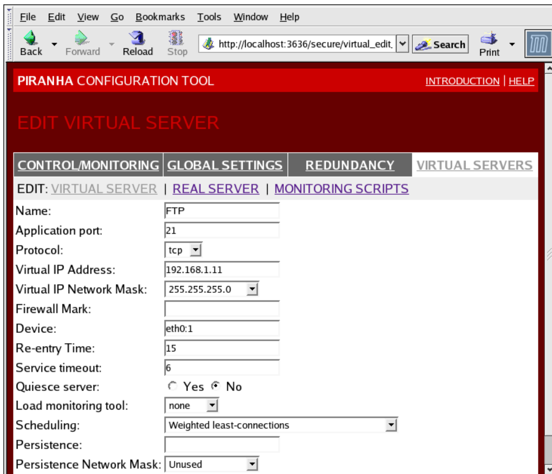
Figure 4.6. The VIRTUAL SERVERS Subsection
